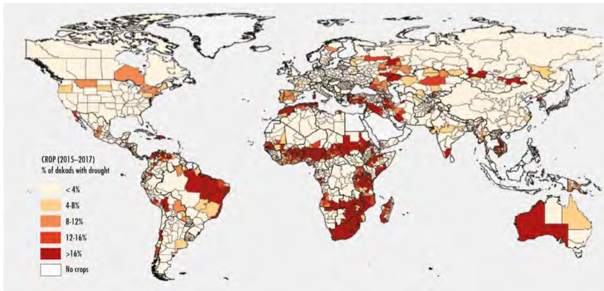
Percentage of time (dekad is a 10-day period) with active vegetation when the Anomaly Hot Spots of Agricultural Production (ASAP) was signaling possible agricultural production anomalies according to NDVI (Normalized Difference Vegetation Index) for more than 25% of the crop areas in 2015–2017 (FAO, IFAD, UNICEF, WFP and WHO, 2018)
