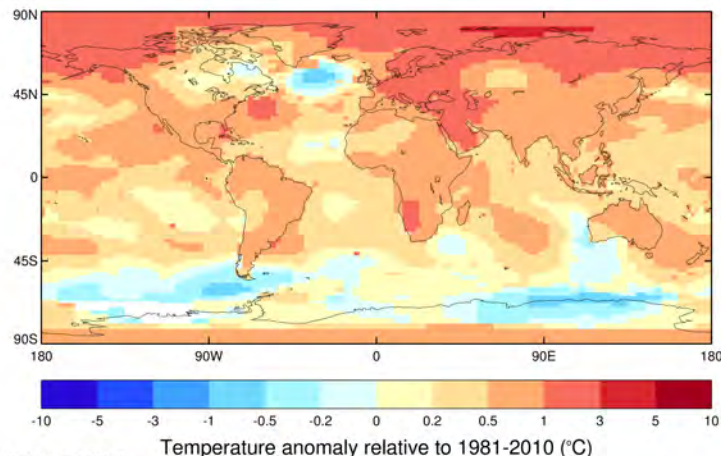
2015-2019 five-year average temperature anomalies relative to the 1981-2010 average. Data are from NASA GISTEMP v4. Data for 2019 to June.
