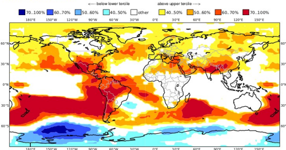
C3S: Météo-France contribution Prob(most likely category of Z500) OND 2022 Nominal forecast start: 01/09/22 Ensemble size = 51, climate size = 600
