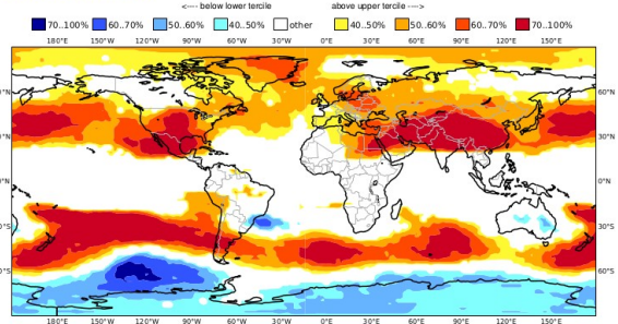
C3S: ECMWF contribution Prob(most likely category of Z500) OND 2022 Nominal forecast start: 01/09/22 Ensemble size = 51, climate size = 600
