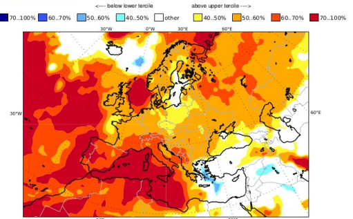
C3S: Météo-France contribution Prob(most likely category of 2m temperature) Nominal forecast start: 01/09/22 Ensemble size = 51, climate size = 600
