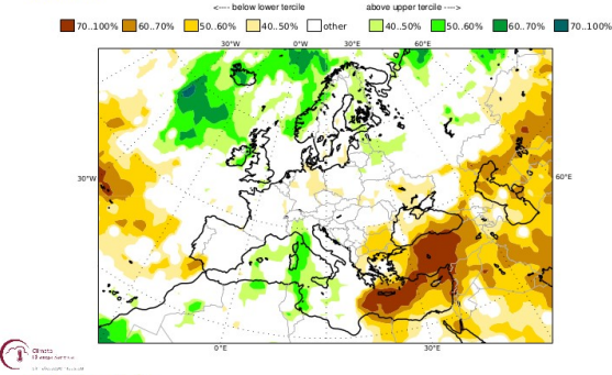
C3S: JMA contribution Prob(most likely category of precipitation) Nominal forecast start: 01/09/22 Ensemble size = 55, climate size = 240
