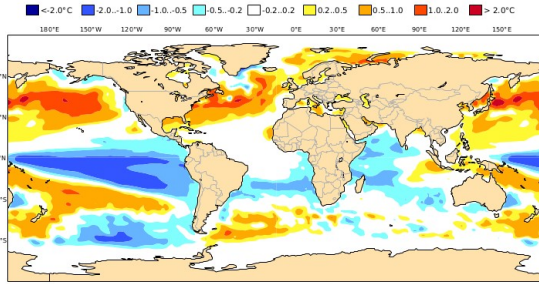
C3S: ECCM contribution Mean SST anomaly Nominal forecast start: 01/09/22 Variance-standardized mean
