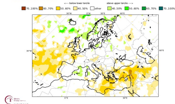
C3S: Météo-France contribution Prob(most likely category of precipitation) Nominal forecast start: 01/09/22 Ensemble size = 51, climate size = 600
