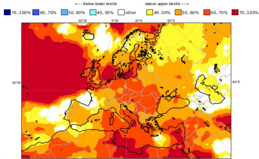
C3S: ECCC contribution Prob(most likely category of 2m temperature) Nominal forecast start: 01/09/22 Unweighted mean
