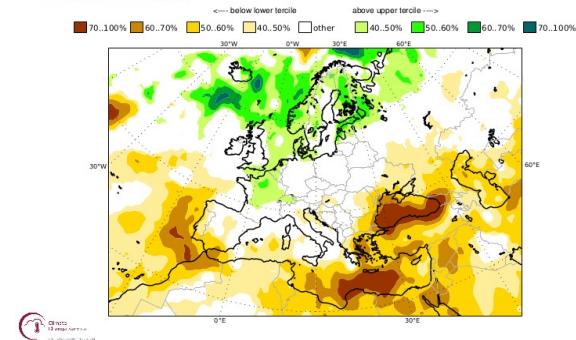
C3S: NCEP contribution Prob(most likely category of precipitation) Nominal forecast start: 01/09/22 Ensemble size = 52, climate size = 384
