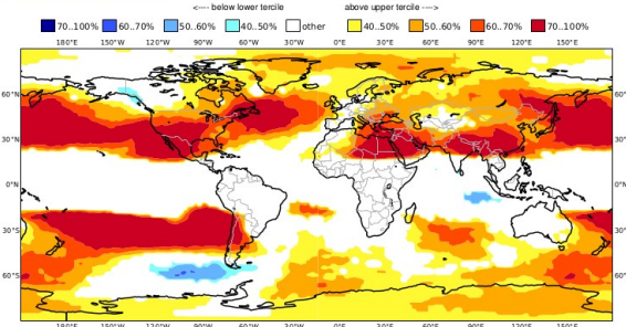
C3S: ECCM contribution Prob(most likely category of Z500) OND 2022 Nominal forecast start: 01/09/22 Unweighted mean
