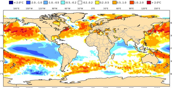
C3S: DWD contribution Mean SST anomaly Nominal forecast start: 01/09/22 Ensemble size = 50, climate size = 720
