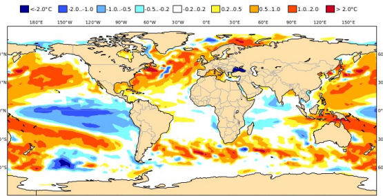
C3S: NCEP contribution Mean SST anomaly Nominal forecast start: 01/09/22 Ensemble size = 52, climate size = 384
