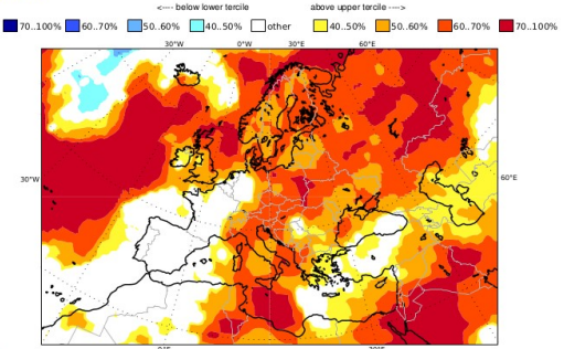
C3S: JMA contribution Prob(most likely category of 2m temperature) Nominal forecast start: 01/09/22 Ensemble size = 55, climate size = 240
