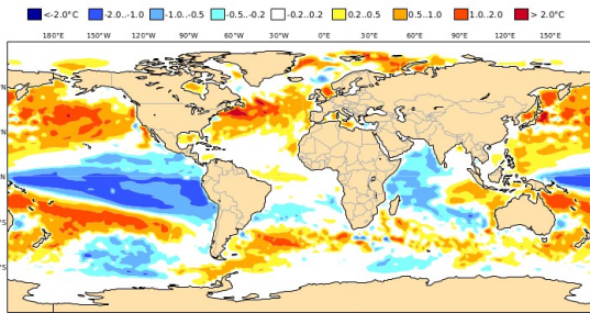
C3S: JMA contribution Mean SST anomaly Nominal forecast start: 01/09/22 Ensemble size = 55, climate size = 240
