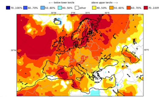
C3S: NCEP contribution Prob(most likely category of 2m temperature) Nominal forecast start: 01/09/22 Ensemble size = 50, climate size = 384
