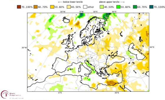
C3S: Met Office contribution Prob(most likely category of precipitation) Nominal forecast start: 01/09/22 Ensemble size = 50, climate size = 672
