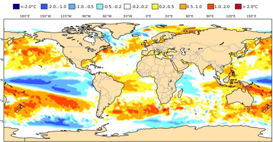
C3S: Météo-France contribution Mean SST anomaly Nominal forecast start: 01/09/22 Ensemble size = 51, climate size = 600
