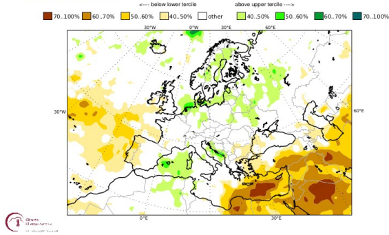
C3S: CMCC contribution Prob(most likely category of precipitation) Nominal forecast start: 01/09/22 Ensemble size = 50, climate size = 960
