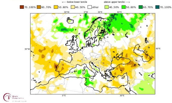
C3S: DWD contribution Prob(most likely category of precipitation) Nominal forecast start: 01/09/22 Ensemble size = 50, climate size = 720
