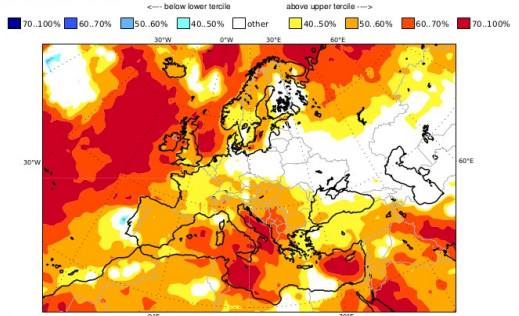
C3S: Met Office contribution Prob(most likely category of 2m temperature) Nominal forecast start: 01/09/22 Ensemble size = 50, climate size = 672
