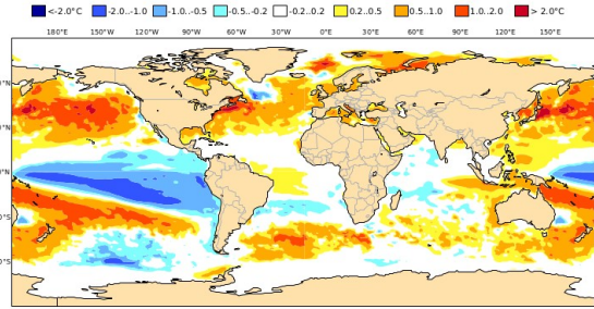
C3S: ECMWF contribution Mean SST anomaly Nominal forecast start: 01/09/22 Ensemble size = 51, climate size = 600
