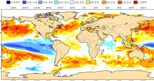
C3S: CMCC contribution Mean SST anomaly Nominal forecast start: 01/09/22 Ensemble size = 50, climate size = 960
