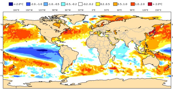
C3S: Met Office contribution Mean SST anomaly Nominal forecast start: 01/09/22 Ensemble size = 50, climate size = 672
