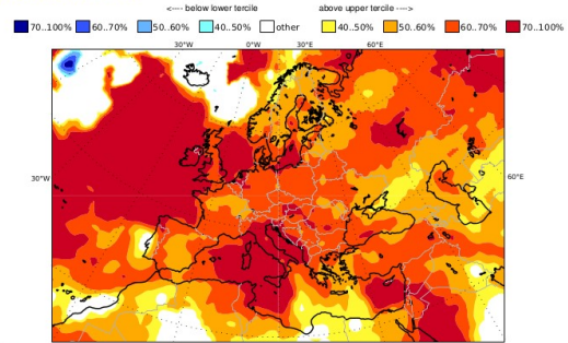
C3S: ECMWF contribution Prob(most likely category of 2m temperature) Nominal forecast start: 01/09/22 Ensemble size = 51, climate size = 600
