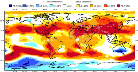
C3S: NCEP contribution Prob(most likely category of Z500) OND 2022 Nominal forecast start: 01/09/22 Ensemble size = 52, climate size = 384
